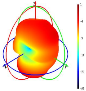
900 MHz
