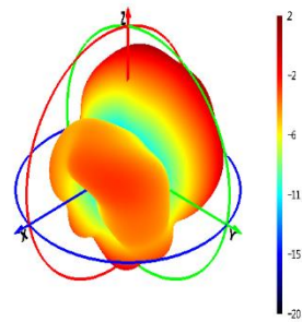
1740 MHz
