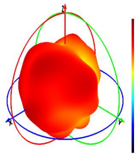
2600 MHz
