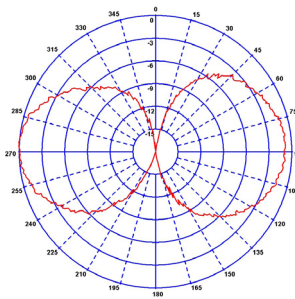
E-Plane (450MHz)
