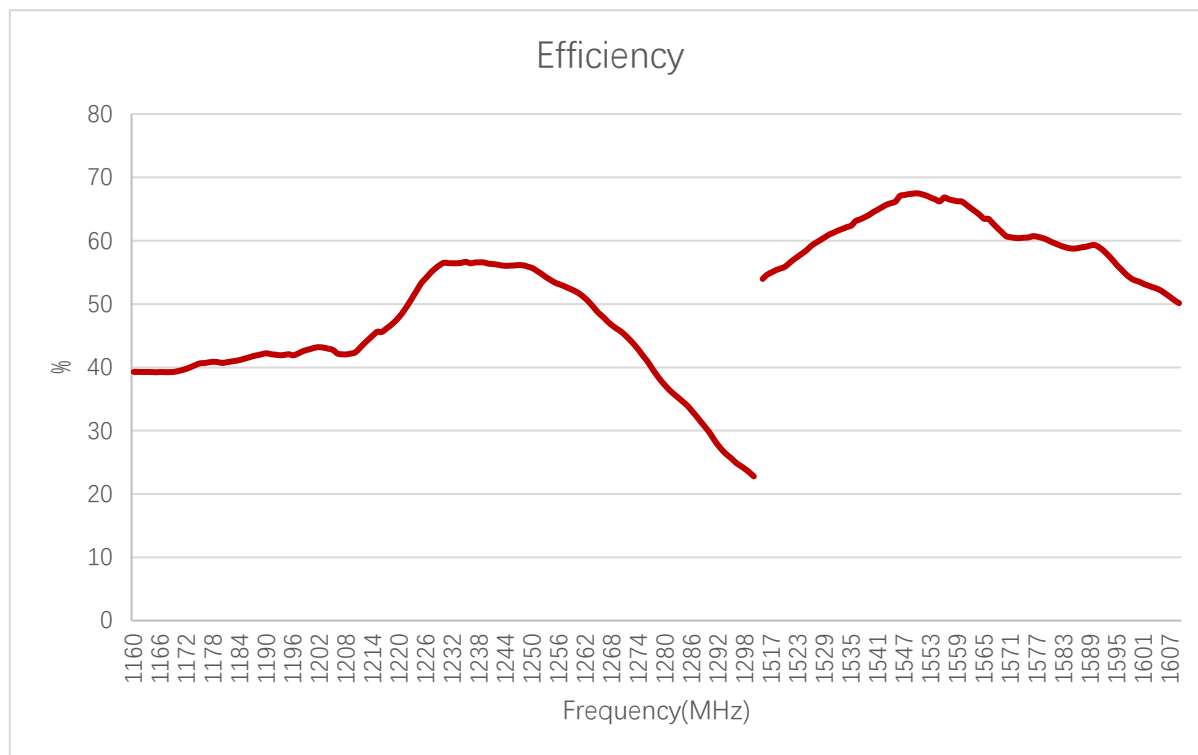
Efficiency (%)
